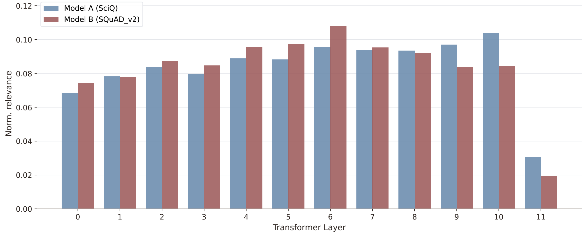
Normalized Per-Layer MLP Relevance
