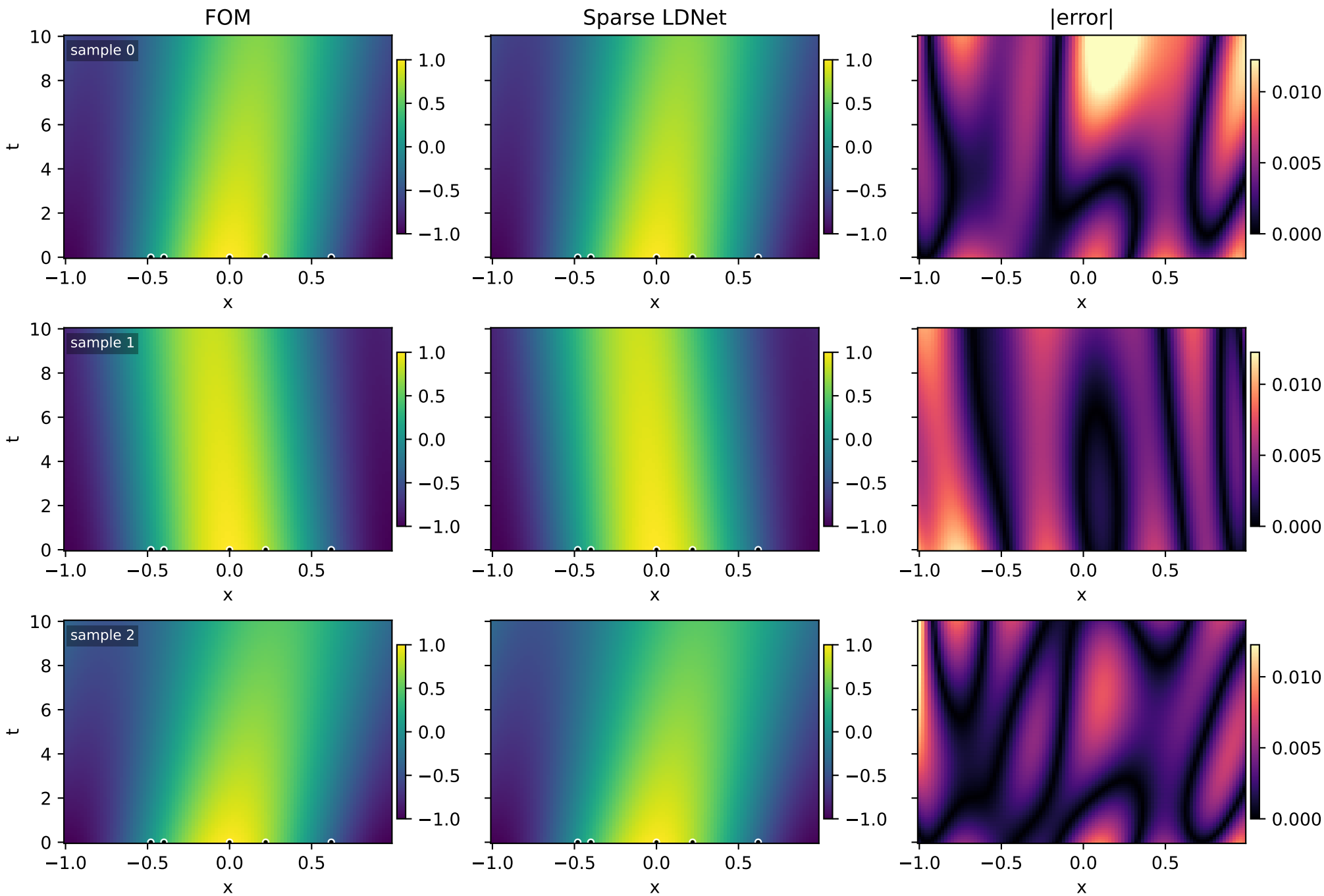
Case 1a sparse encoder, sensor ratio=0.05, NRMSE=2.573e-03
