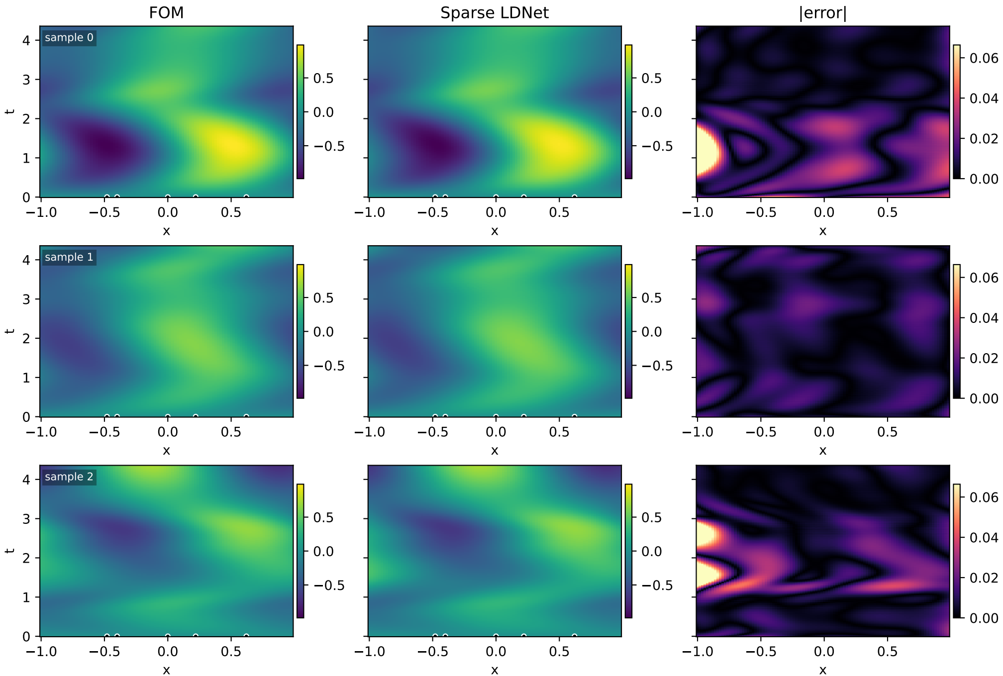
Case 1b sparse encoder, sensor ratio=0.05, NRMSE=1.014e-02
