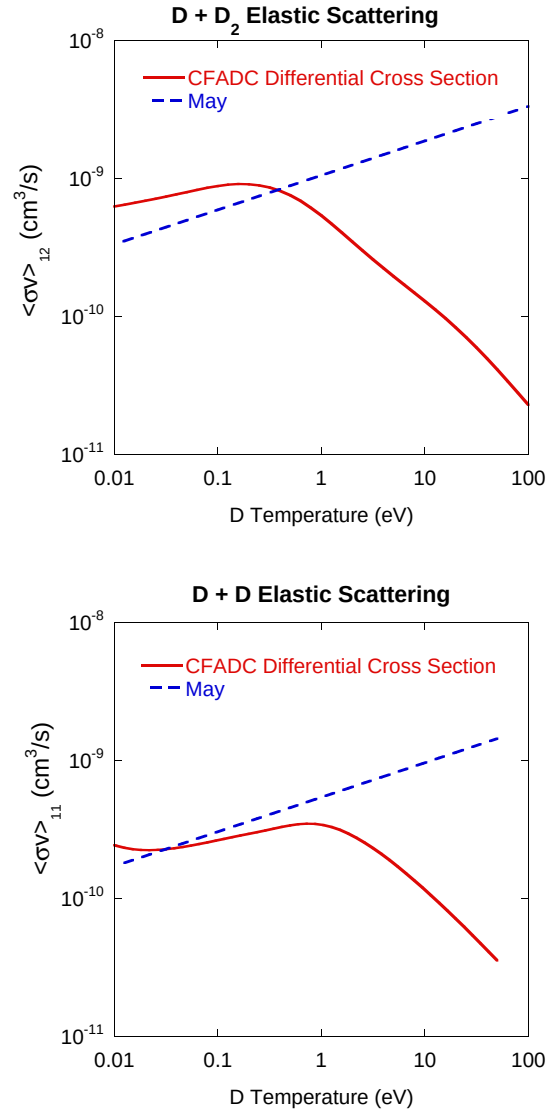
Figure 2.9: Comparison of reaction rates for the D + D_2 and D + D systems. The original rates suggested by May[36] and effective rates computed from the CFADC data are shown.
