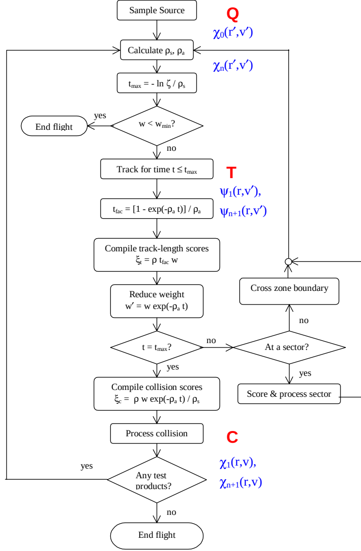
Figure 2.3: Flow chart of DEGAS 2 subroutine follow, showing the steps involved in tracking a flight from its birth to its termination. Note the weight reduction, and collision and tracklength estimators (Sec. 2.3). The operators from the integral equations are shown along with the pre- and post-collision densities. These labels tie the practical algorithmic operations to the equations in Sec. 2.2.3. Some details have been omitted for clarity.
