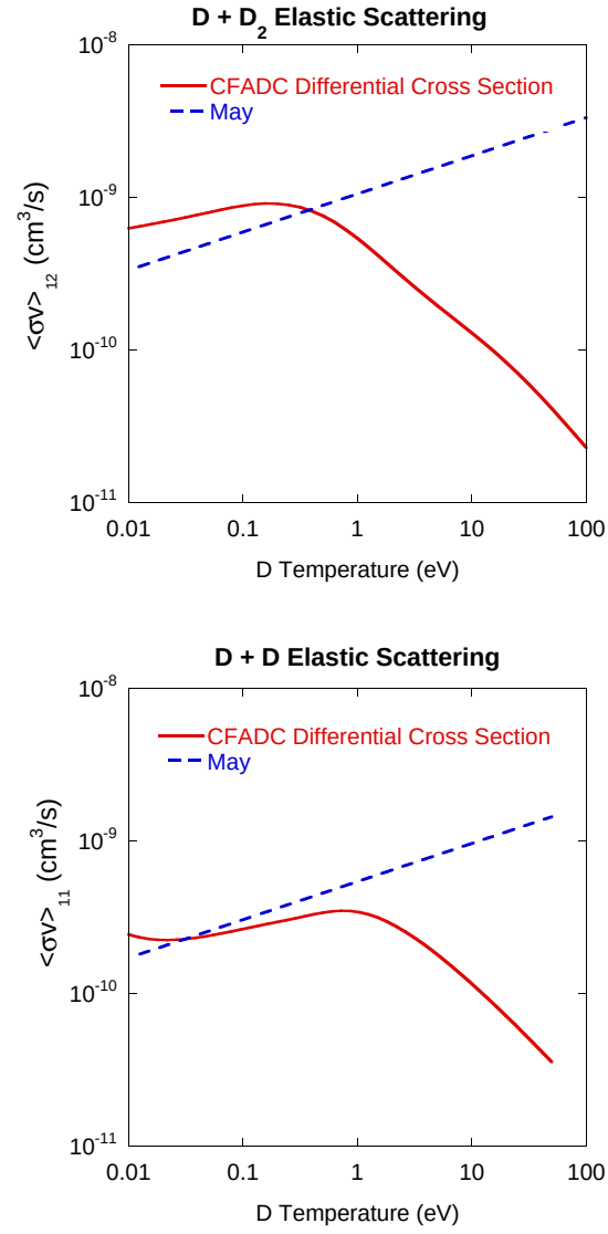
Figure 2.9: Comparison of reaction rates for the D + D_2 and D + D systems. The original rates suggested by May[34] and effective rates computed from the CFADC data are shown.
