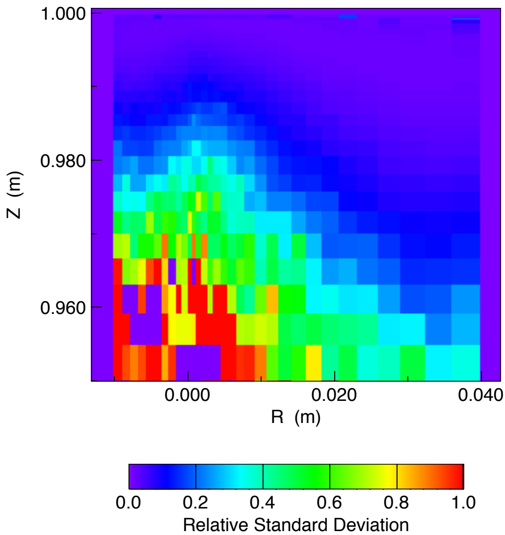
D+ Source Relative Standard Deviation - No Ionization Suppression
