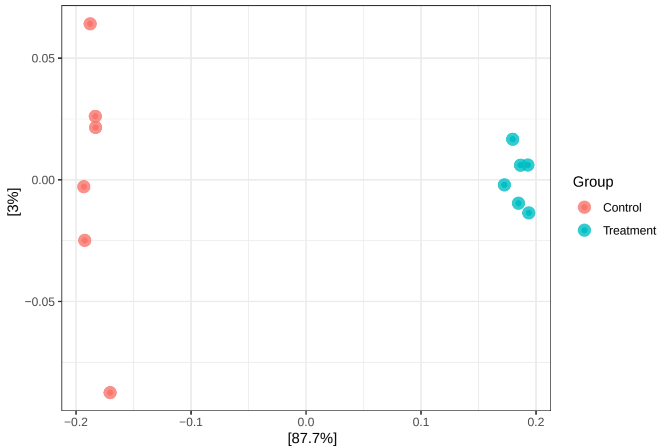
PCoA Ordination (Bray–Curtis Distance)
