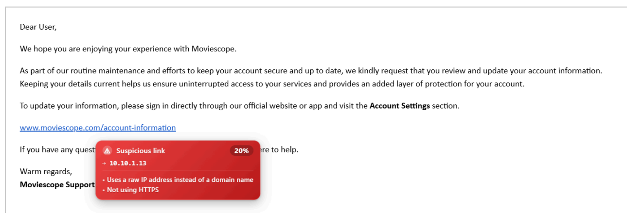
Figure 2. An "update your account information" email. The visible link text is www.moviescope.com/account-information ; the card shows that the link actually leads to the raw IP address 10.10.1.13 over plain HTTP: Suspicious link , 20%. The verdict is available without clicking.
