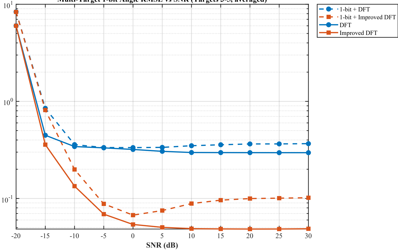
Multi-Target 1-bit Angle RMSE vs SNR (Targets 3-5, averaged)
