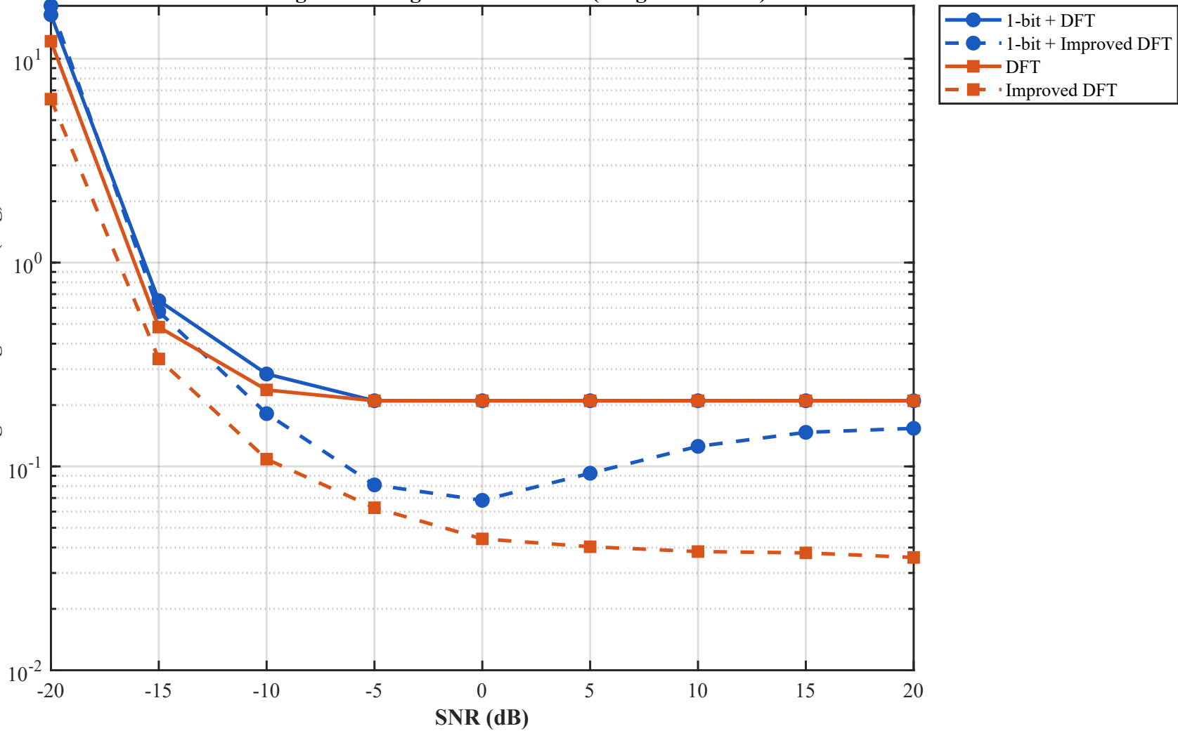
Multi-Target 1-bit Angle RMSE vs SNR (Target 4 at 18.0^\circ )
