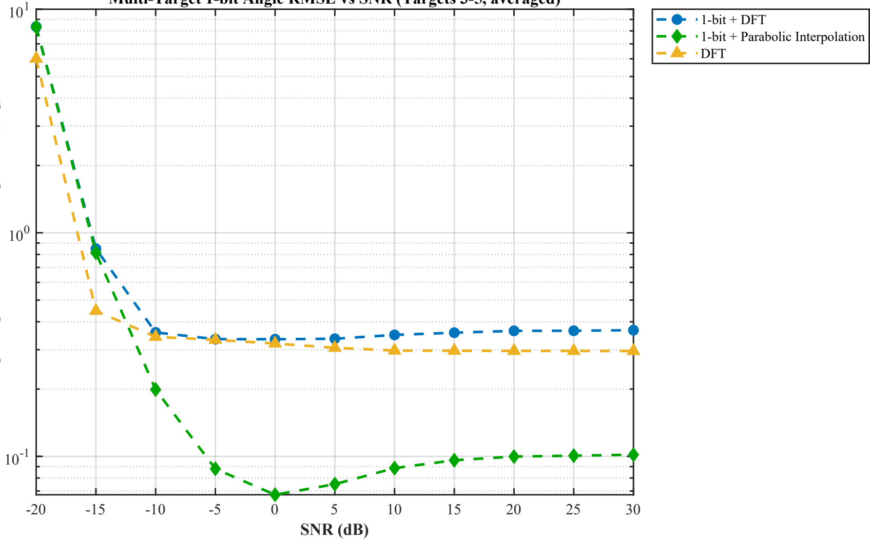
Multi-Target 1-bit Angle RMSE vs SNR (Targets 3-5, averaged)
