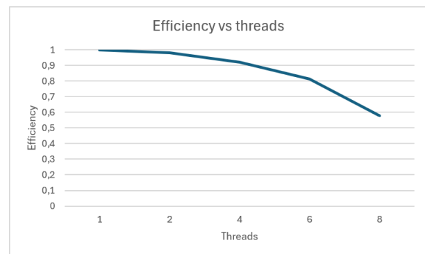
Figure 6: Parallel efficiency on the 8000 × 8000 grid.
