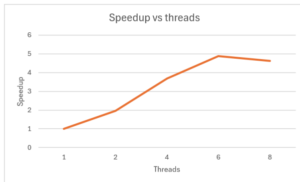
Figure 5: Speedup curve on the 8000 × 8000 grid.
