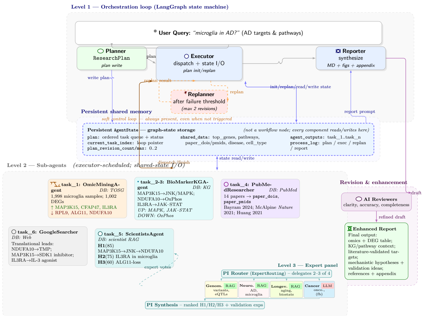
Figure 1: OmniCellAgent three-level hierarchy organised around a shared memory. Top - Level 1 (orchestration loop): User Query → Planner → Executor → Reporter, with the query anchored at the top-left of the full orchestration lane and the Executor containing an internal judgment node that routes success to the next task and failures to the Replanner. In the LangGraph implementation, the Planner produces the ResearchPlan and writes it into persistent AgentState ; the Executor then reads the current task from state and delegates it to the appropriate Level 2 agent. Middle - Persistent shared memory (blue band): plan, current_task_index, shared_data (top_genes, pathways, paper_dois/pmids, disease, cell_type), agent_outputs, and process_log; every component reads and writes here, so this band is the single coordination point between the loop, the sub-agents, and the revision module. Bottom-left - Level 2 (representative scheduled sub-agents): a representative six-task AD run — task_1 OmicMining (DEGs), task_2-3 BioMarkerKG (pathways), task_4 PubMedResearcher (paper DOIs), task_5 ScientistsAgent (ranked hypotheses), task_6 GoogleSearcher (translational leads). Following the LangGraph implementation, Level 2 is shown as an executor-scheduled block with one bidirectional control link from the Executor into the task block and one bidirectional read/write link to AgentState ; peer-to-peer agent wiring is omitted because coordination happens through the shared state rather than direct agent chaining. Level 3 (expert panel) is its own teal box and feeds task_5 via a dashed "expert votes" arrow, showing that the Scientists agent is itself a panel of Genomics / Neuroscience / Longevity experts. Bottom-right - Revision & enhancement (violet): the Reporter draft is passed to the AI Reviewers for clarity, accuracy, and completeness, then the refined draft becomes the Enhanced Report - the final output of the system.
