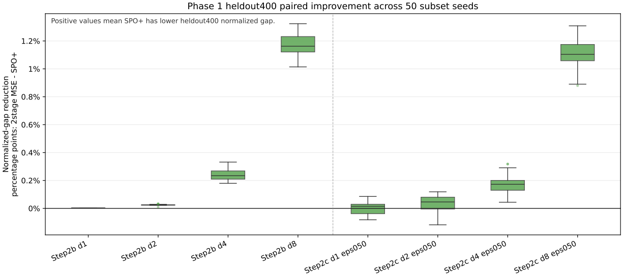
Figure 5: Paired heldout400 improvement: 2stage gap minus SPO+ gap.
