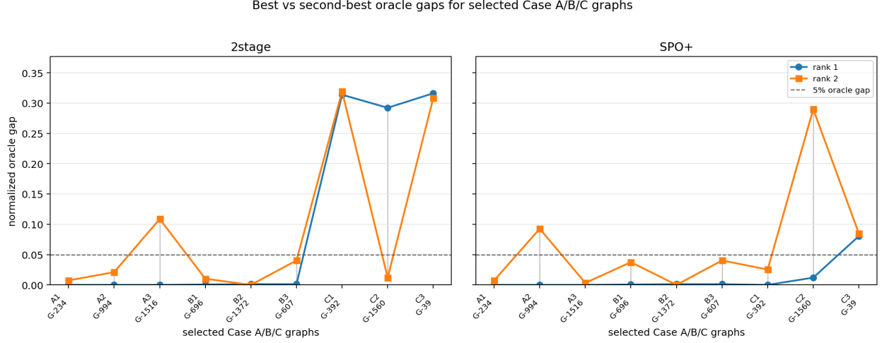
Figure 12: Rank-1 and rank-2 normalized oracle gaps for the selected Case A/B/C graphs.
