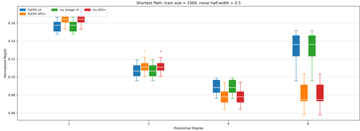
Figure 2: Shortest-path fixed-data comparison, train size 1000 and noise half-width 0.5.
