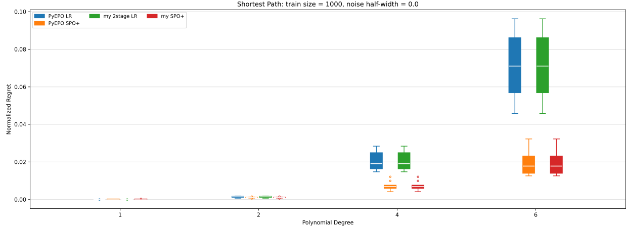
Figure 1: Shortest-path fixed-data comparison, train size 1000 and noise half-width 0.0.
