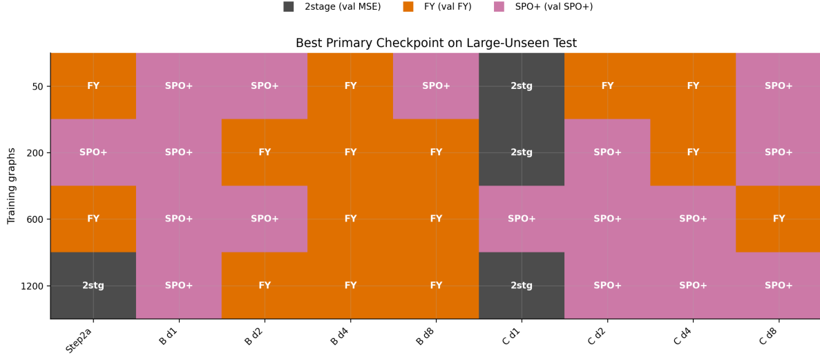
Figure 6: Best primary checkpoint map on unseen10000. The x-axis is label regime, and the y-axis is train size. Each cell reports the primary checkpoint with the lowest mean normalized decision gap among 2stage, FY selected by validation FY loss, and SPO+ selected by validation SPO+ loss. Cell color and text identify the winner. Lower gap is better; this map asks which method wins in each regime-size setting.
