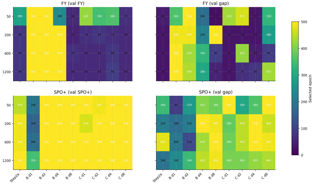
Figure 10: Selected checkpoint epochs. The x-axis is label regime, the y-axis is train size, and panels correspond to FY selected by validation FY loss, FY selected by validation decision gap, SPO+ selected by validation SPO+ loss, and SPO+ selected by validation decision gap. Cell color and text report selected epoch. The figure asks whether selectors choose early or late checkpoints, which is important because FY and SPO+ may have different training dynamics.
