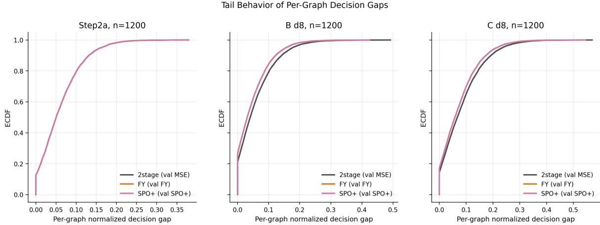
Figure 14: Tail behavior of per-graph normalized decision gaps. The x-axis is per-graph normalized decision gap, the y-axis is the empirical CDF, and colors indicate primary checkpoint families. Panels show representative regimes. Lower gaps are better; curves shifted left suggest better tail and overall per-graph performance. The figure asks whether FY/SPO+ reduce hard-case gaps rather than only improving the mean.
