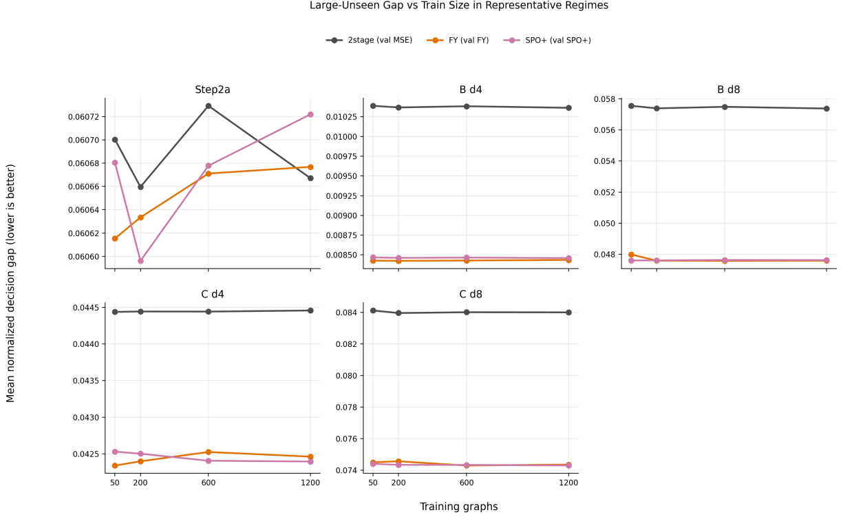
Figure 7: Large-unseen normalized gap versus train size for representative regimes. The x-axis is the number of training graphs, and the y-axis is mean normalized decision gap, where lower is better. Lines correspond to 2stage, FY selected by validation FY loss, and SPO+ selected by validation SPO+ loss. Panels show Step2a, Step2b d4/d8, and Step2c d4/d8. The figure asks whether the decision-focused advantage persists across train sizes rather than only after averaging over n .
