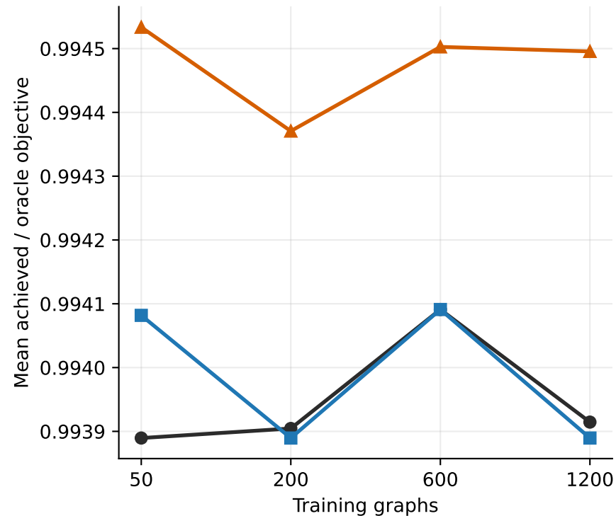
Held-out noisy-linear test 400 graphs
