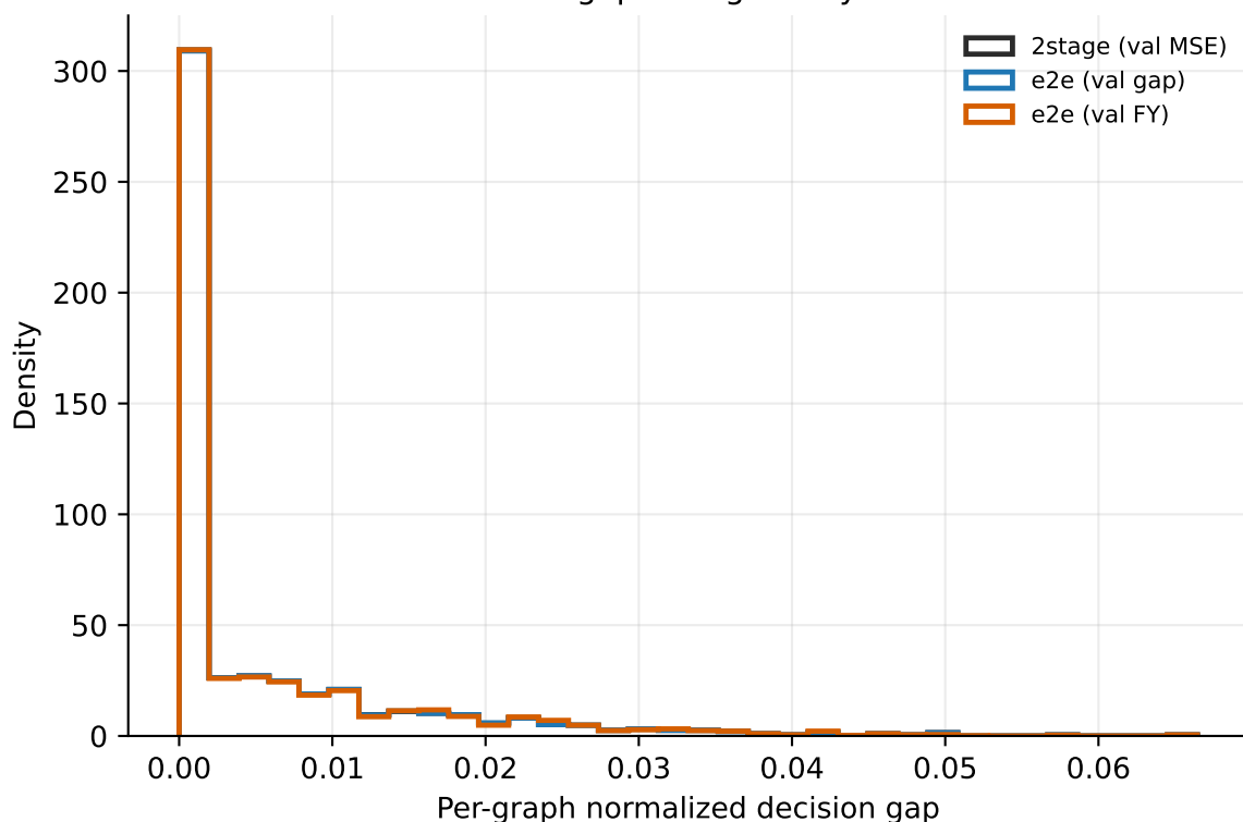
E2E val-gap vs val-FY checkpoints
