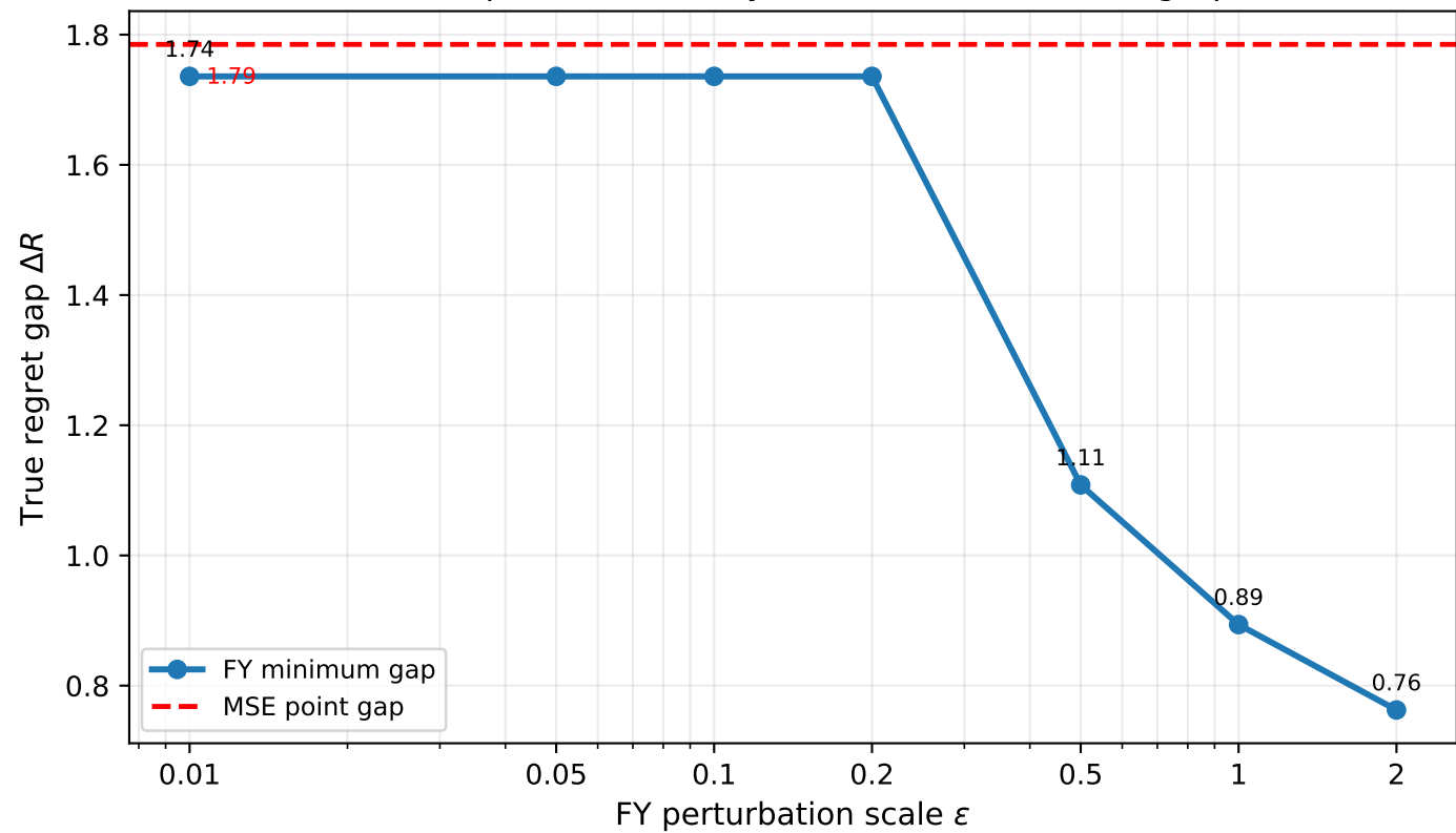
Plot-level epsilon sensitivity ( \hat{w}_e = \theta_1 u_e + \theta_2 c_e , 100 graphs)
