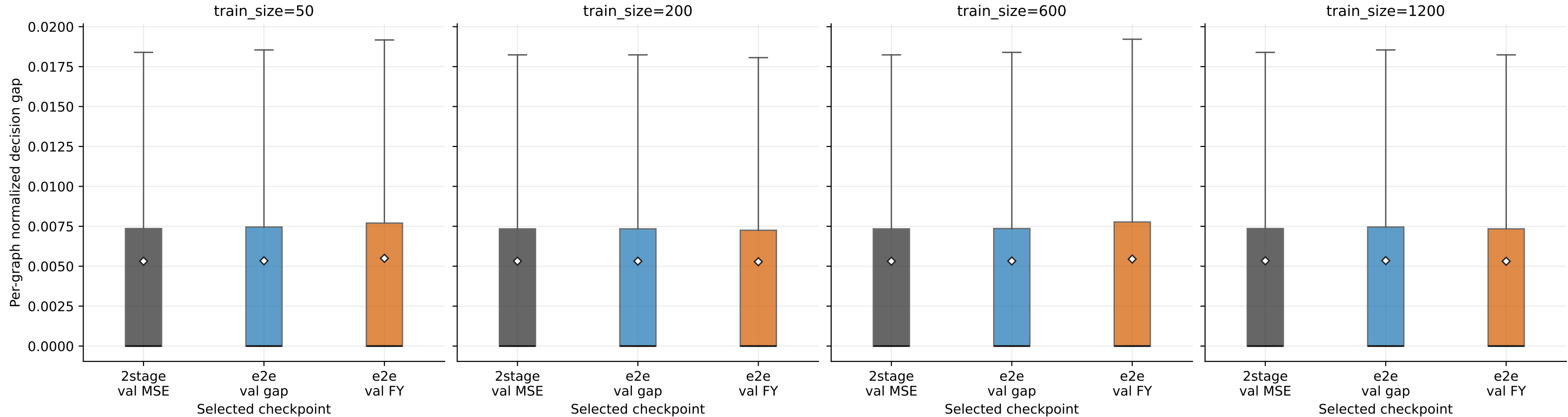
Unseen noisy-linear test Per-graph Gap Distribution (1000 graphs)
