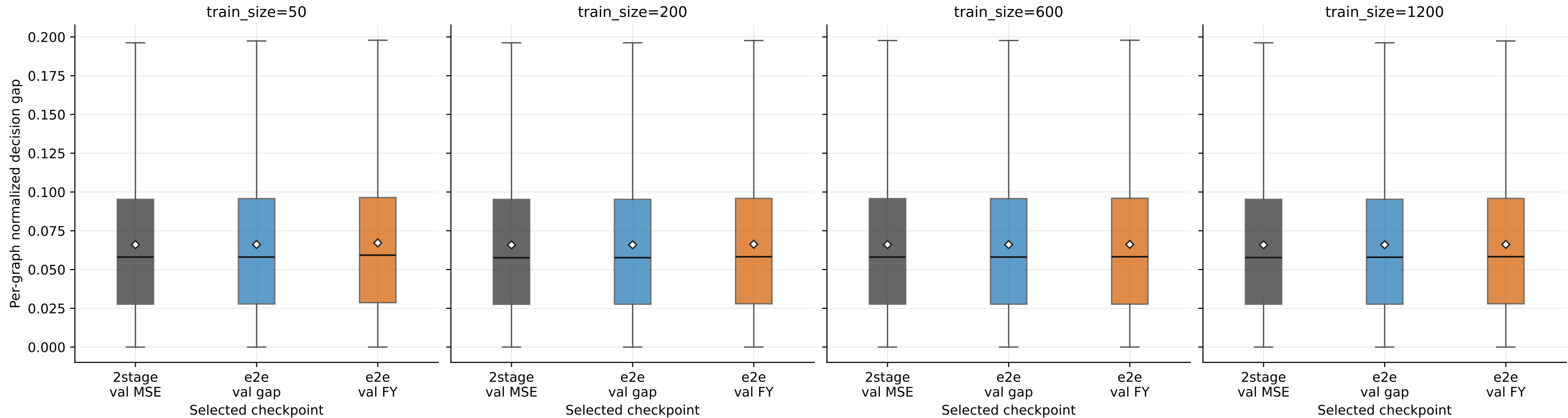
Realistic-synthetic stress test Per-graph Gap Distribution (2000 graphs)
