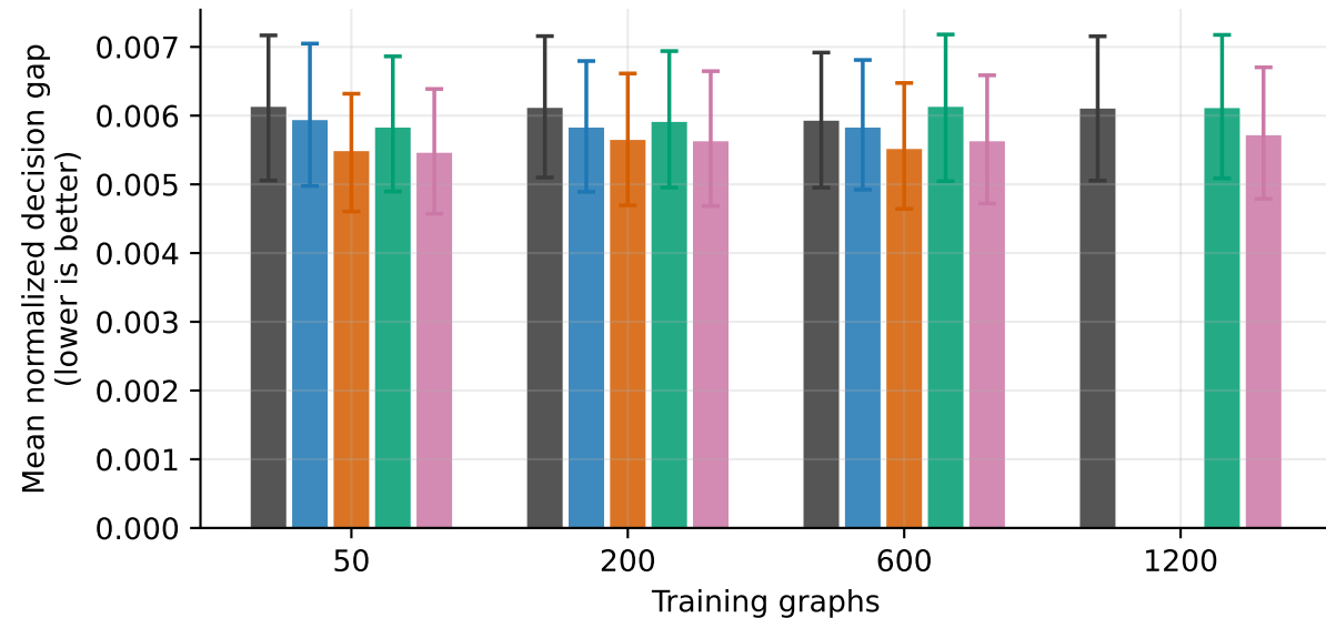
Held-out noisy-linear test 400 graphs
