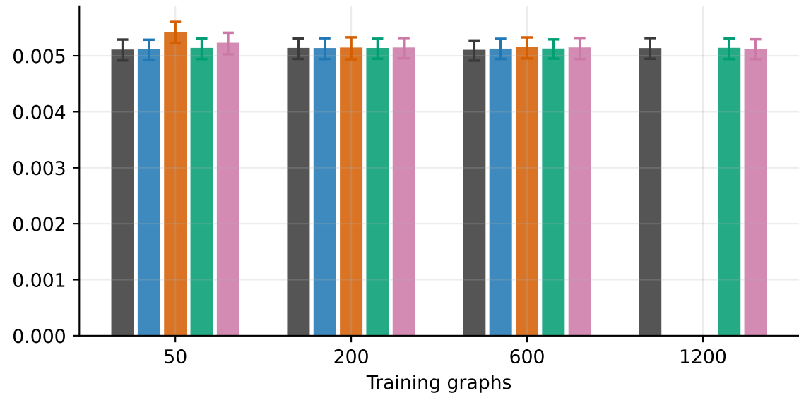
Unseen noisy-linear test 10000 graphs
