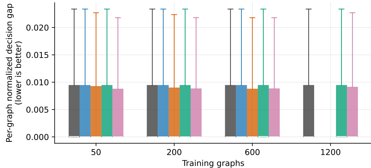
Held-out noisy-linear test 400 graphs
