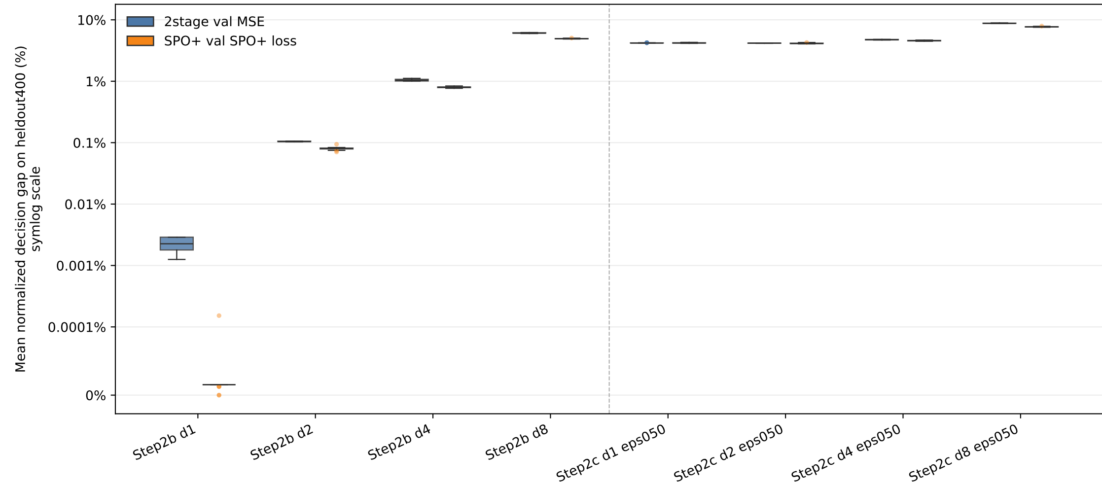
Phase 1 heldout400 decision gap (%) across 50 subset seeds
