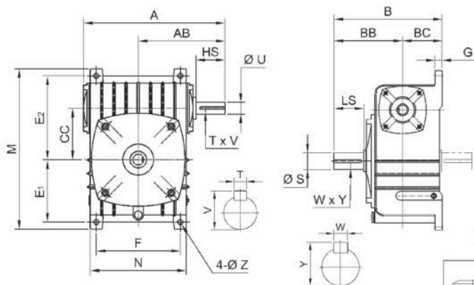
MCX Shaft Direction
