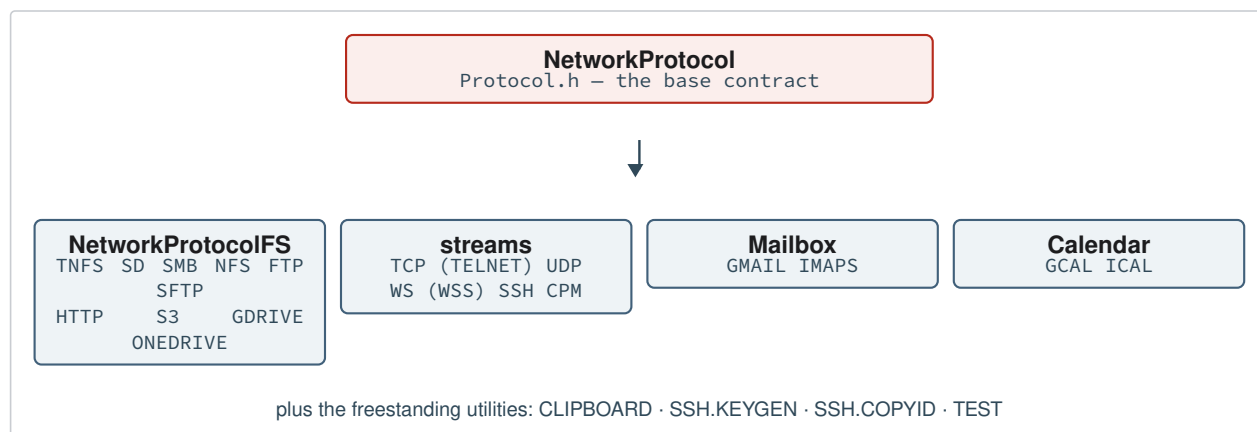
Figure 2. The class families in lib/network-protocol . TELNET subclasses TCP; WSS subclasses WS; the mail and calendar bases do the heavy lifting for their providers.
