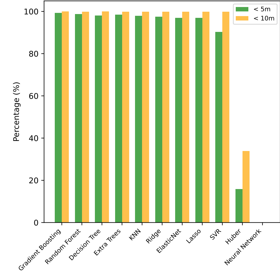
Accuracy Thresholds
