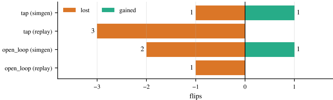
cyberrag B3_DIRECT_QUERY: stability flips (threshold=0.7)
