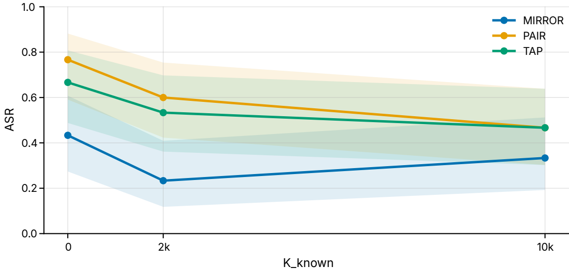
GeneralRAG B1_TEXT_POISON Patched-KnownSet
