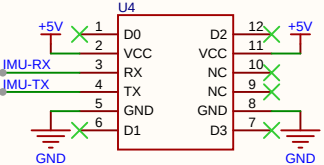
IMU-姿态检测模块
