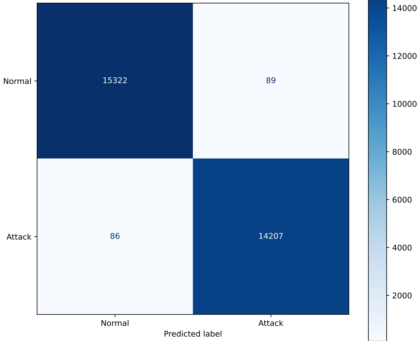
Confusion Matrix — Decision Tree (No PCA)
