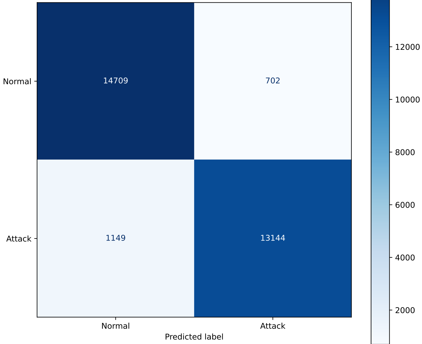
Confusion Matrix — Logistic Regression (No PCA)
