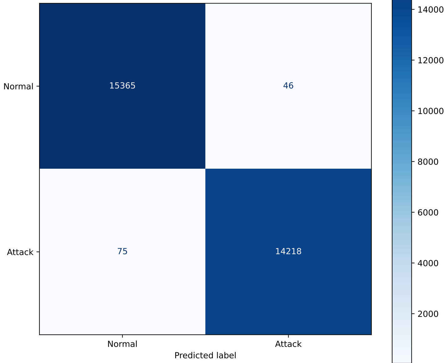
Confusion Matrix — Random Forest (No PCA)
