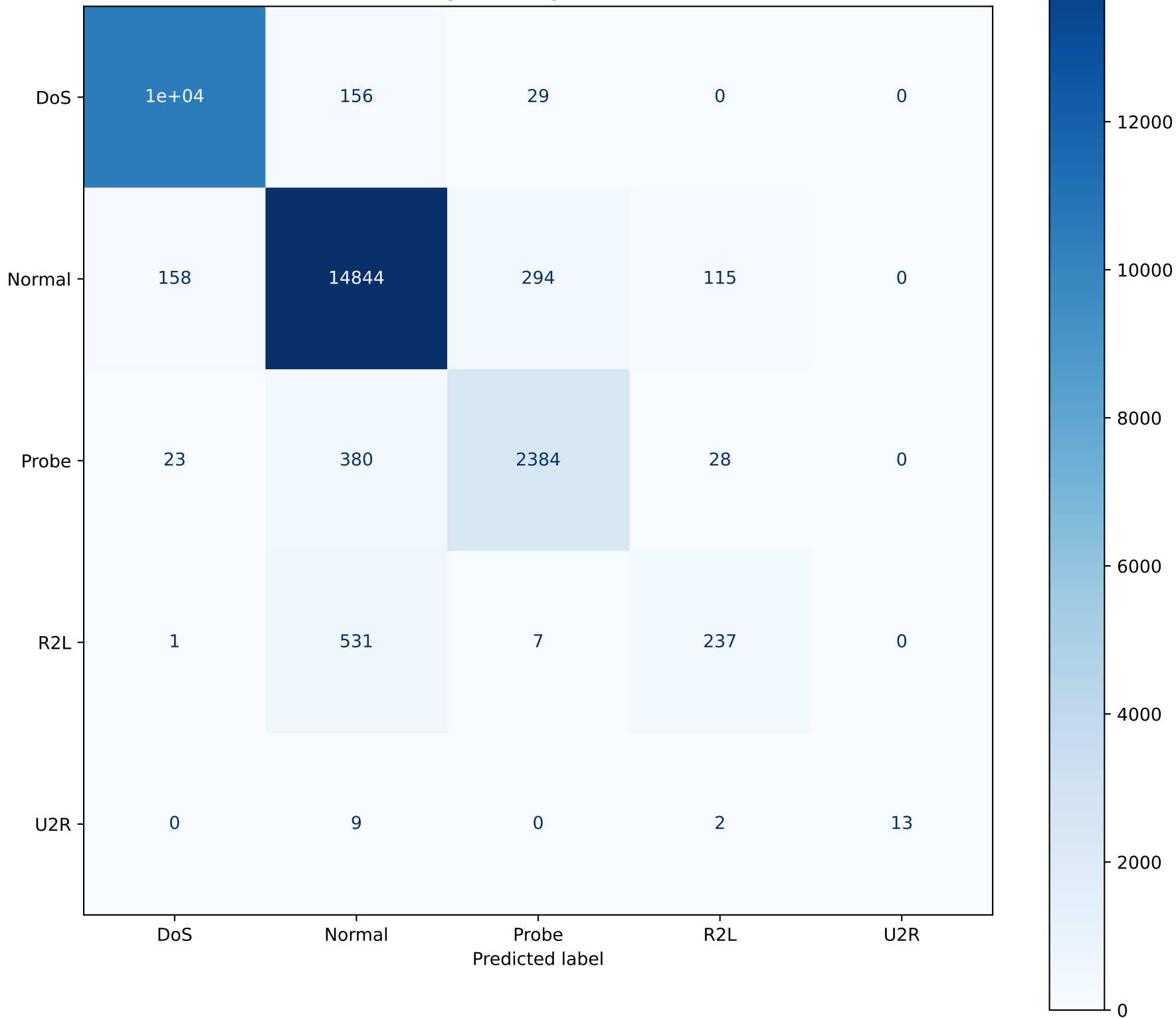
Confusion Matrix — Logistic Regression (Multiclass, No PCA)
