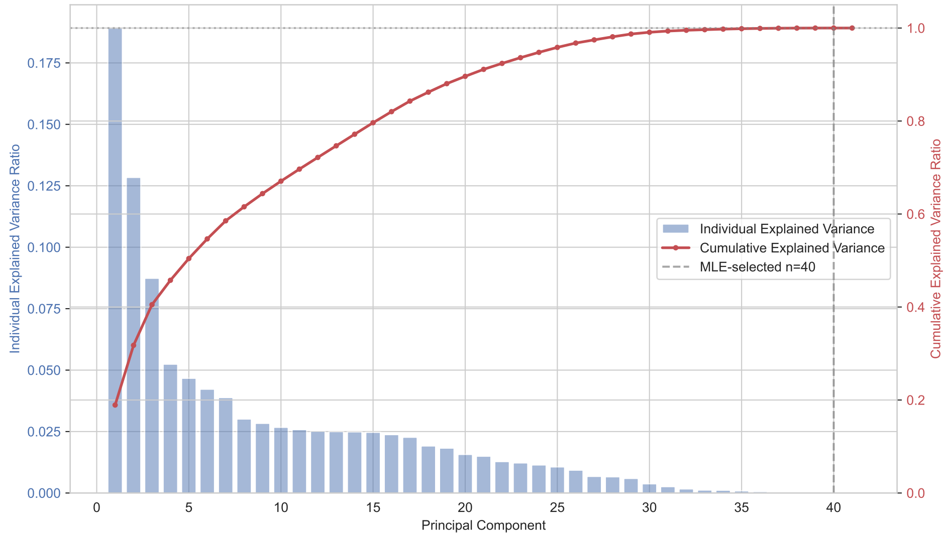
PCA Scree Plot — Individual &amp; Cumulative Explained Variance
