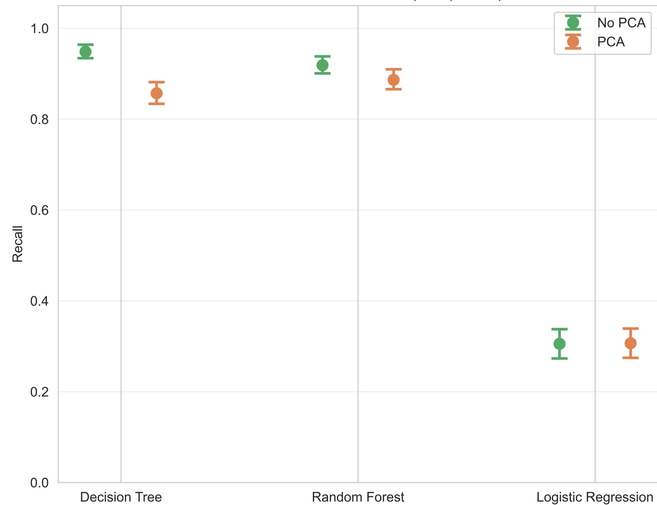
R2L Recall — 95% Bootstrap CI (n=776)
