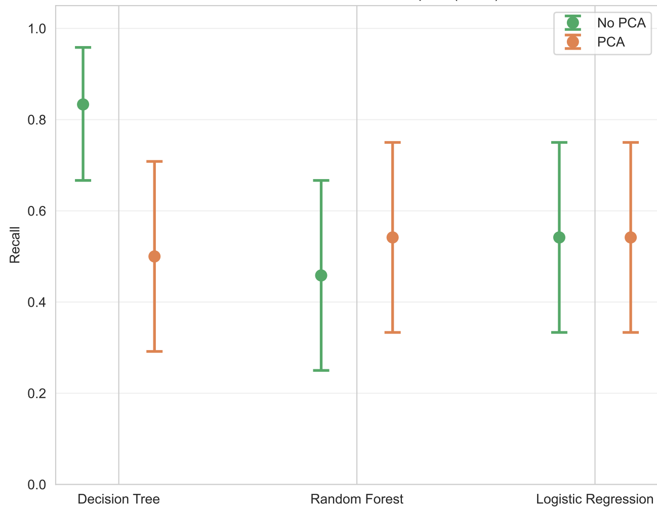
U2R Recall — 95% Bootstrap CI (n=24)
