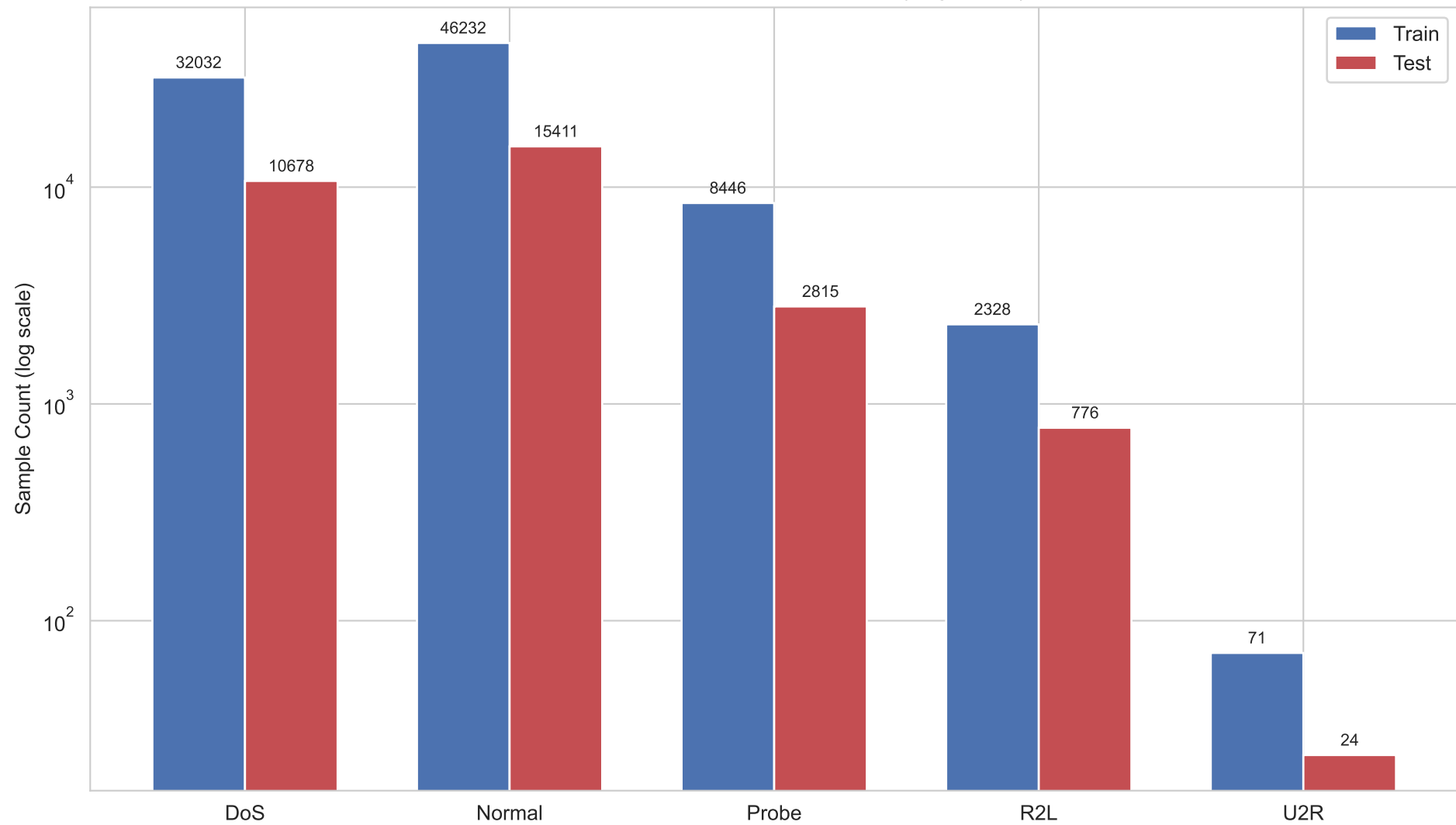
Class Distribution — Train vs Test (Log Scale)
