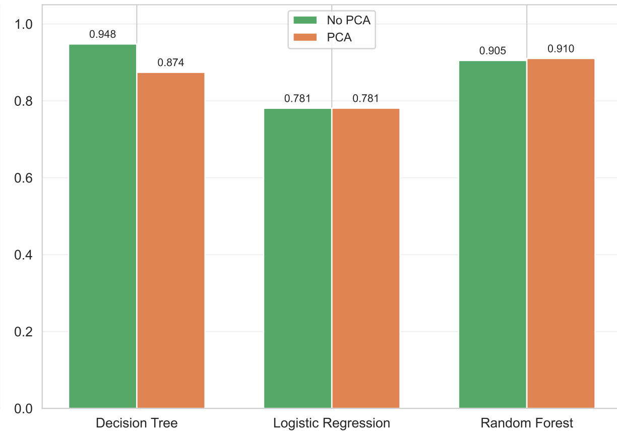
R2L Recall
