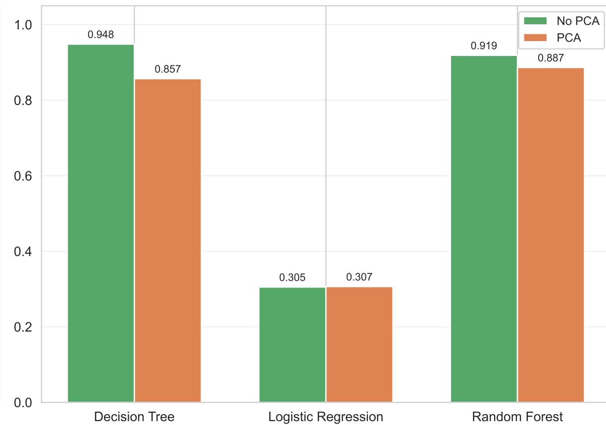
R2L Recall
