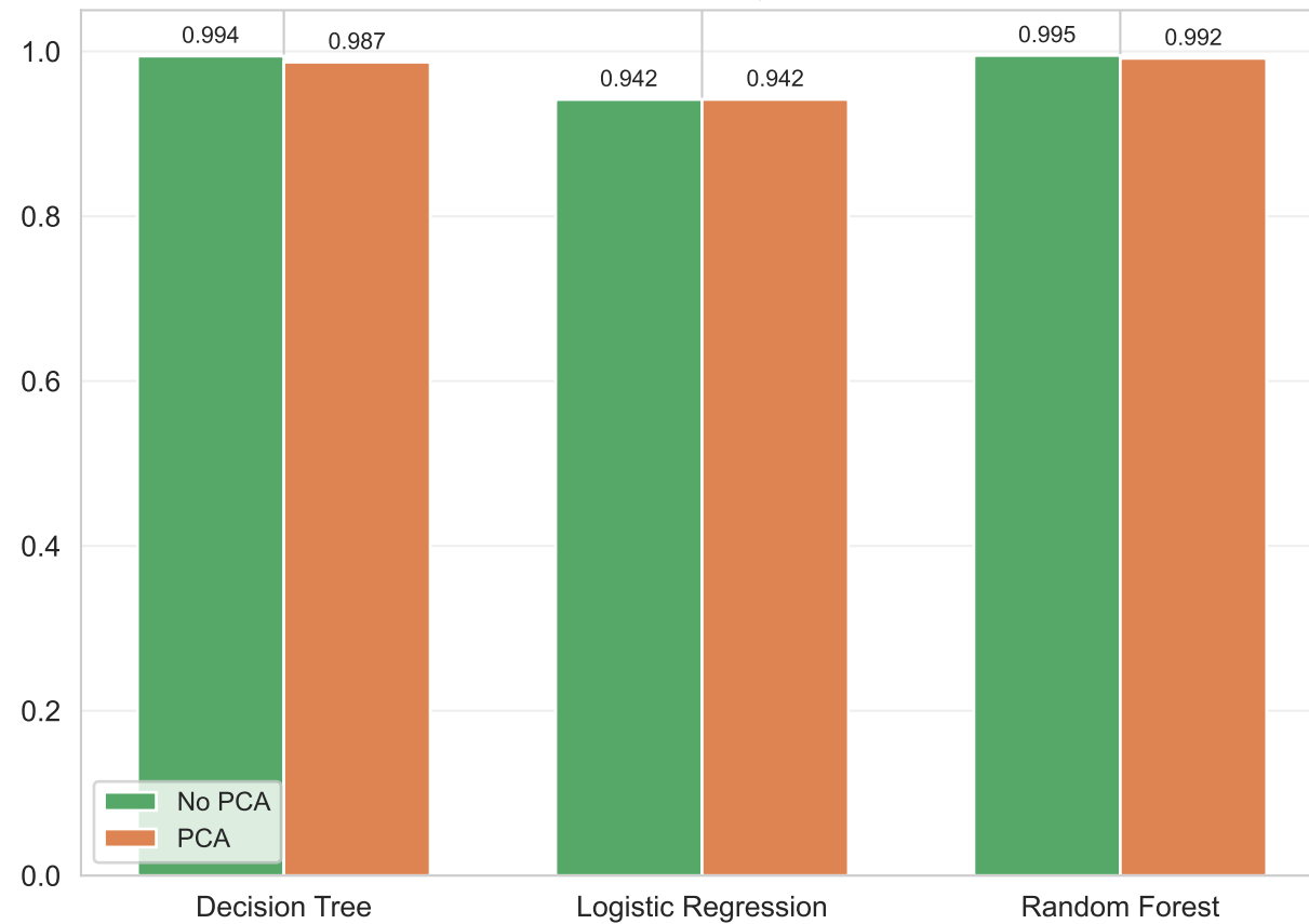
U2R Recall
