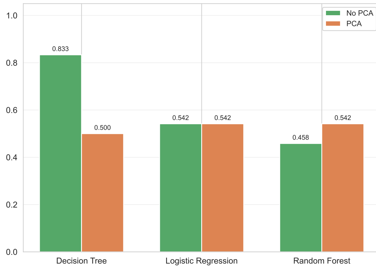
U2R Recall
