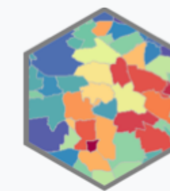
rgdal
