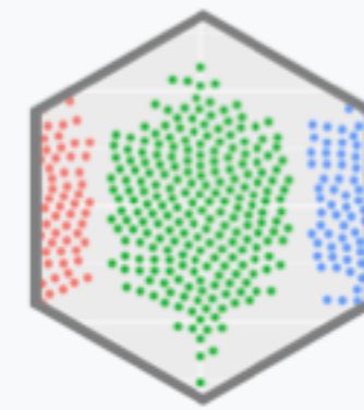
ggbeeswarm
