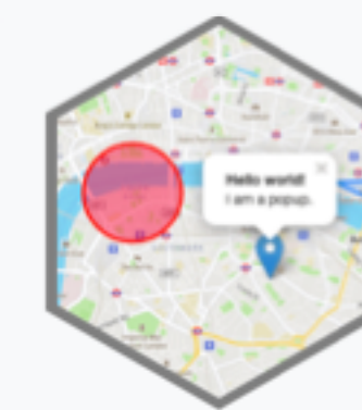
leaflet
