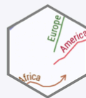
geomtextpath
