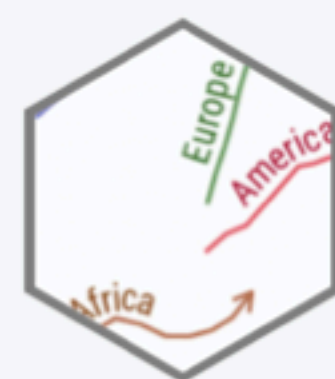
geomtextpath
