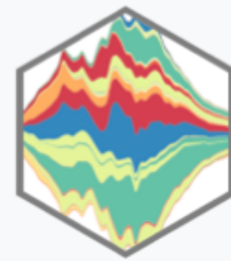
streamgraph
