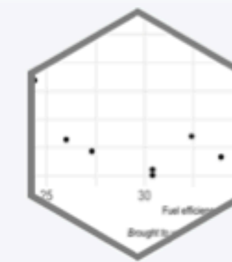
hrbrthemes
