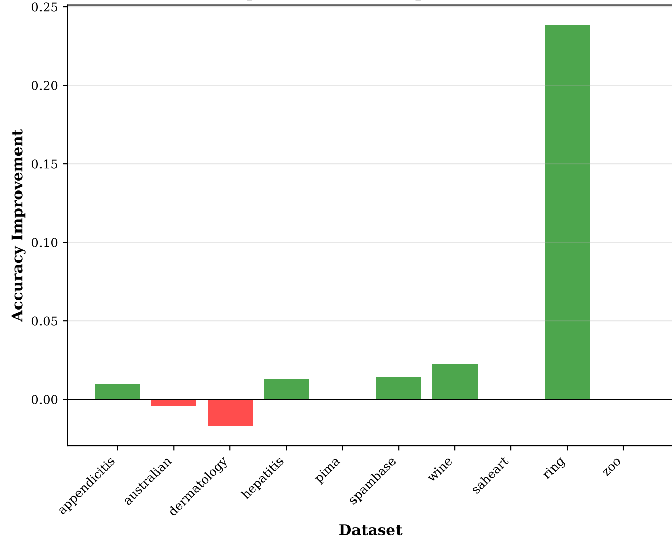
Impact of Partition Optimization
