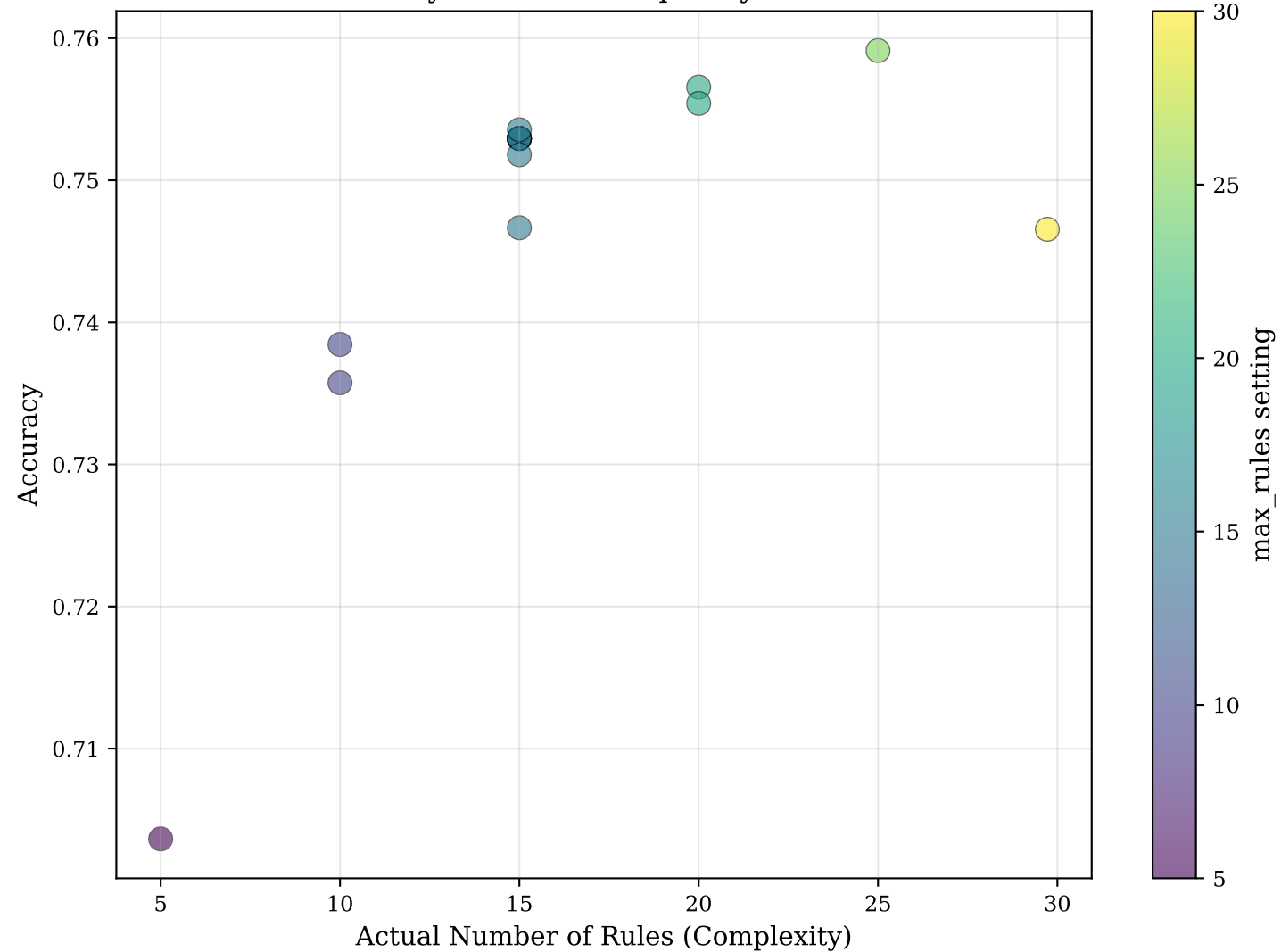
Accuracy vs Model Complexity Trade-off
