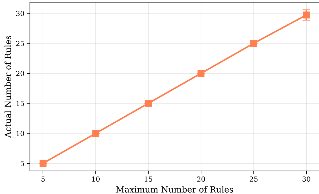
Impact of max_rules on Model Complexity
