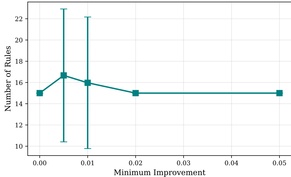
Impact of min_improvement on Model Complexity
