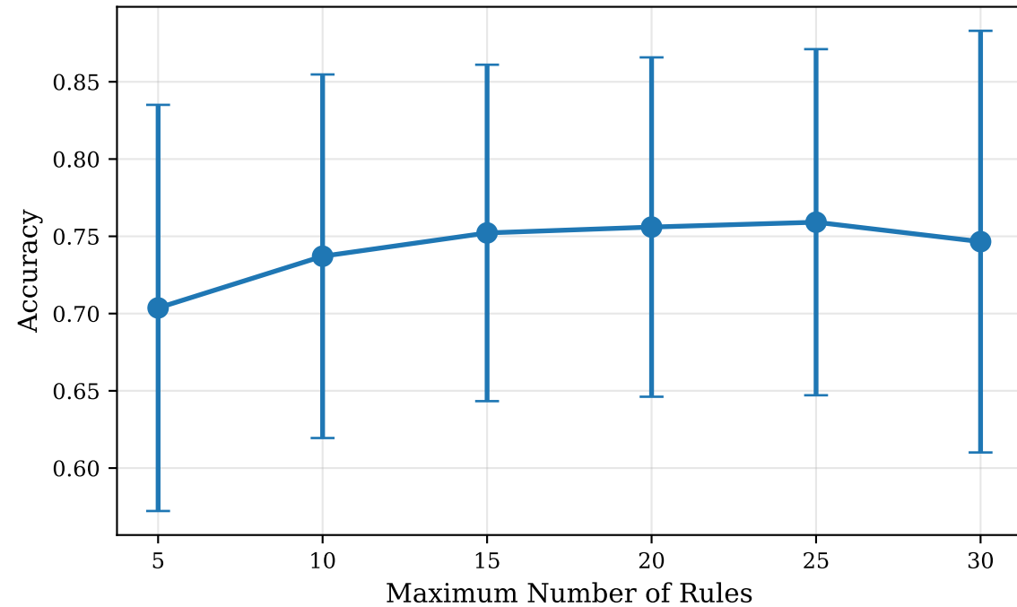
Impact of max_rules on Accuracy
