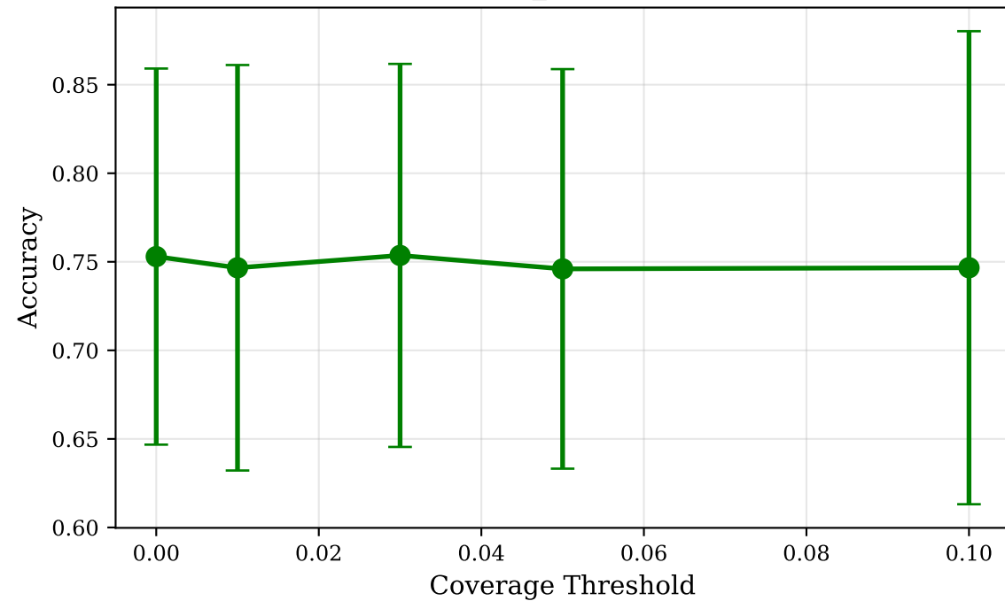
Impact of coverage_threshold on Accuracy
