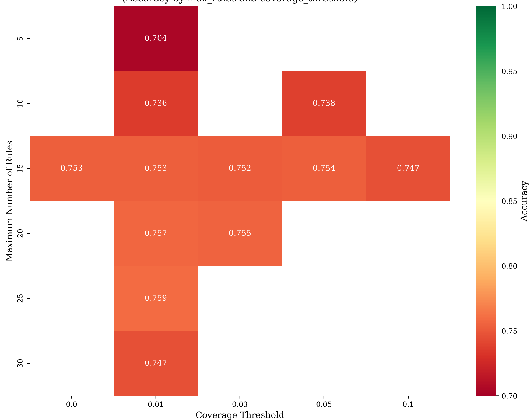
Configuration Performance Heatmap (Accuracy by max_rules and coverage_threshold)
