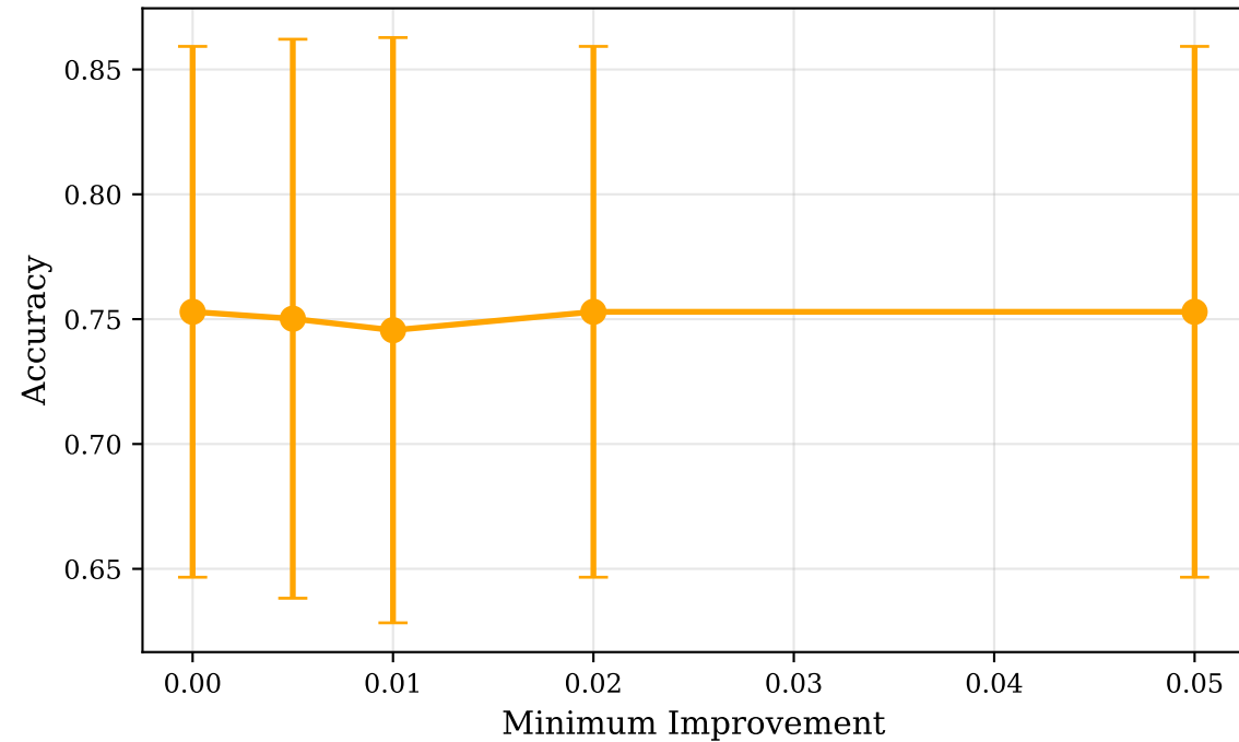
Impact of min_improvement on Accuracy
