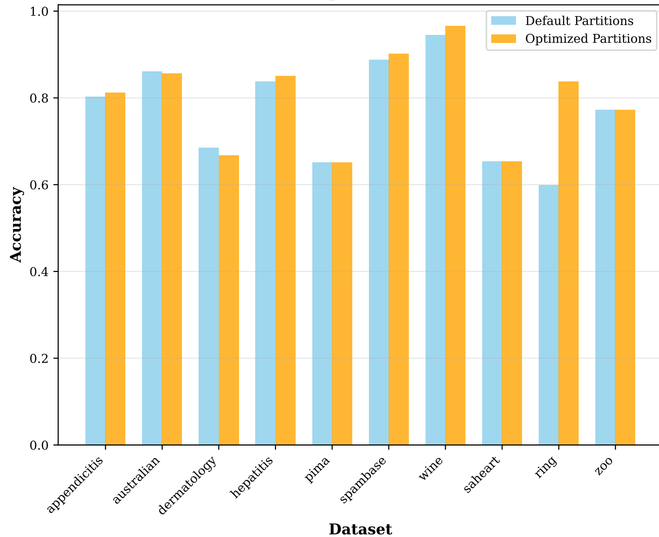
Default vs Optimized Partitions
