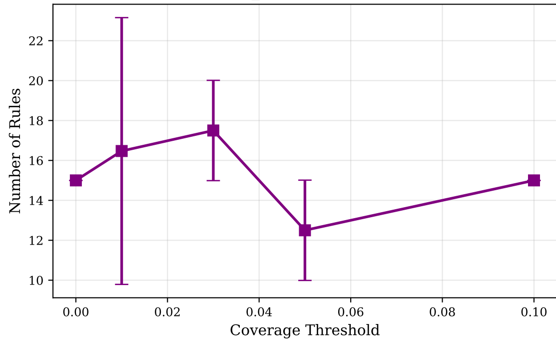
Impact of coverage_threshold on Model Complexity
