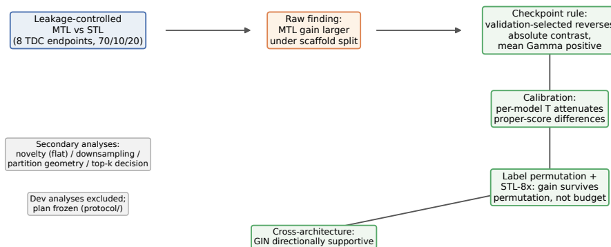
Fig. 1 Study design and principal diagnostic findings. Main evidential chain (top): leakage-controlled MTL vs. STL comparison reveals a raw gain that is larger under scaffold-grouped evaluation; checkpoint selection reverses the absolute contrast while preserving a positive mean protocol interaction; strict same-model temperature calibration attenuates the gain to near zero; label-permuted and compute-matched controls show the gain survives full label permutation and is not reproduced by additional single-task updates; a matched-scale GIN sensitivity reproduces the positive direction. Secondary analyses (grey): novelty dependence, downsampling, partition-geometry reweighting, and decision-level analysis.
