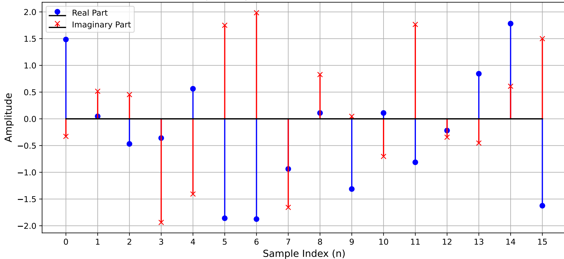
Input Signal: Time Domain (N=16)
