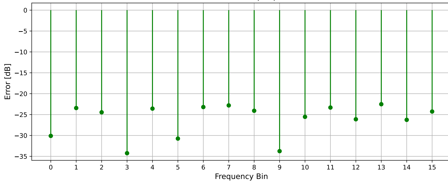
Error Plot (dB)
