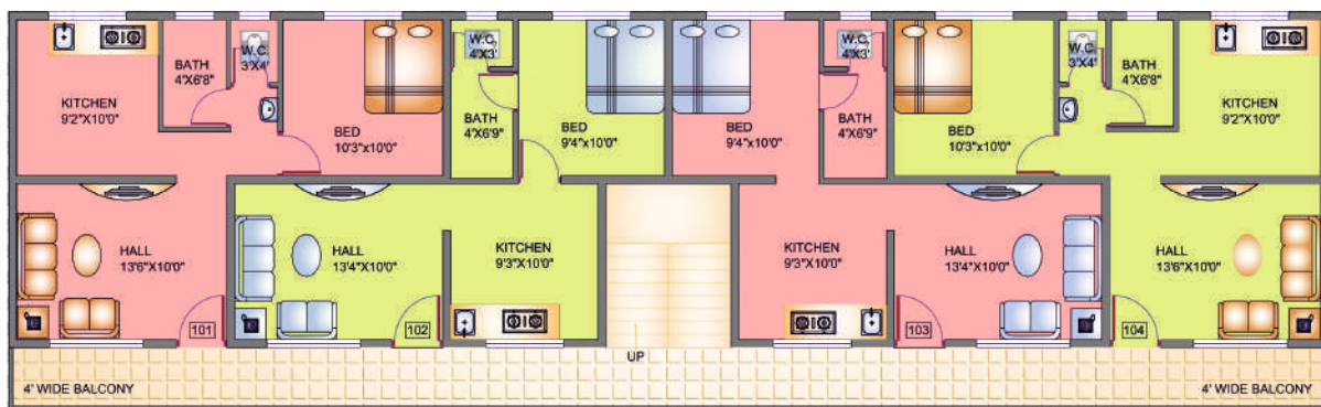
First Floor Plan - 1 BHK
