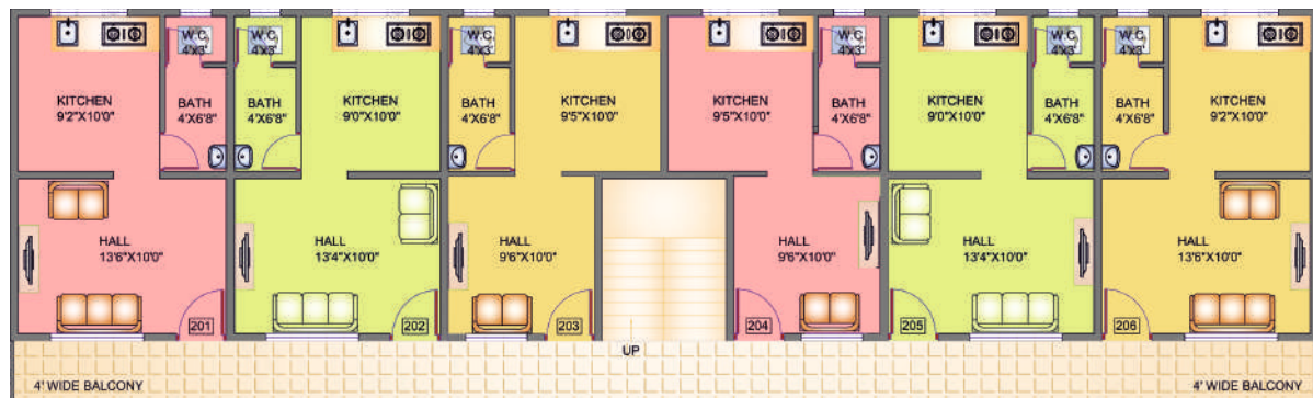
Second Floor Plan - 1 RK
