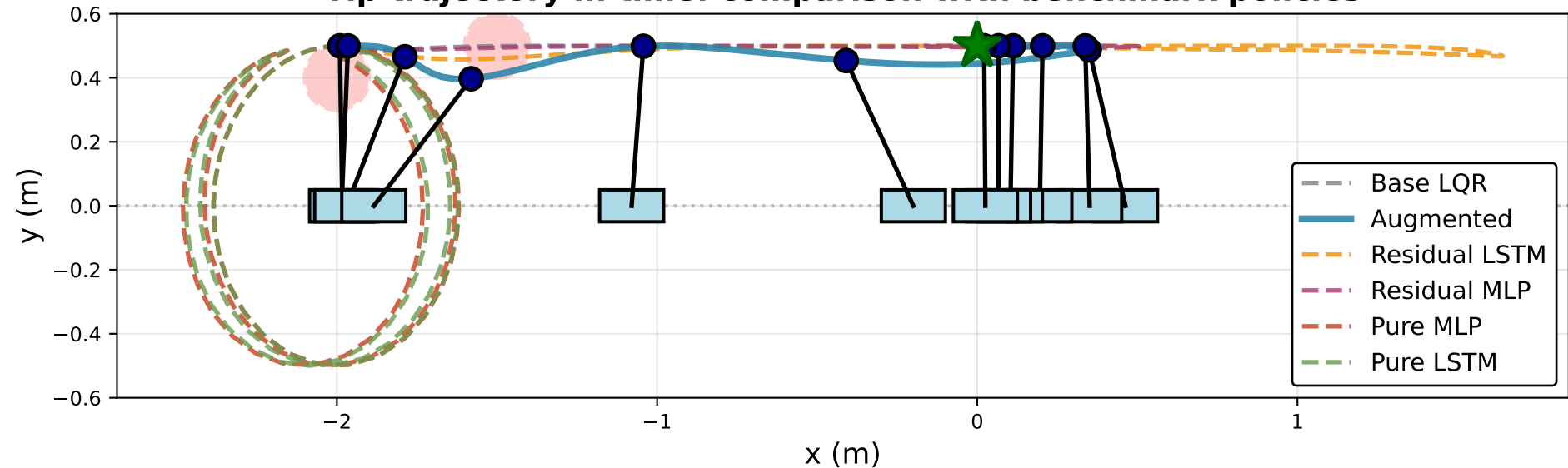
Tip trajectory in time: comparison with benchmark policies
