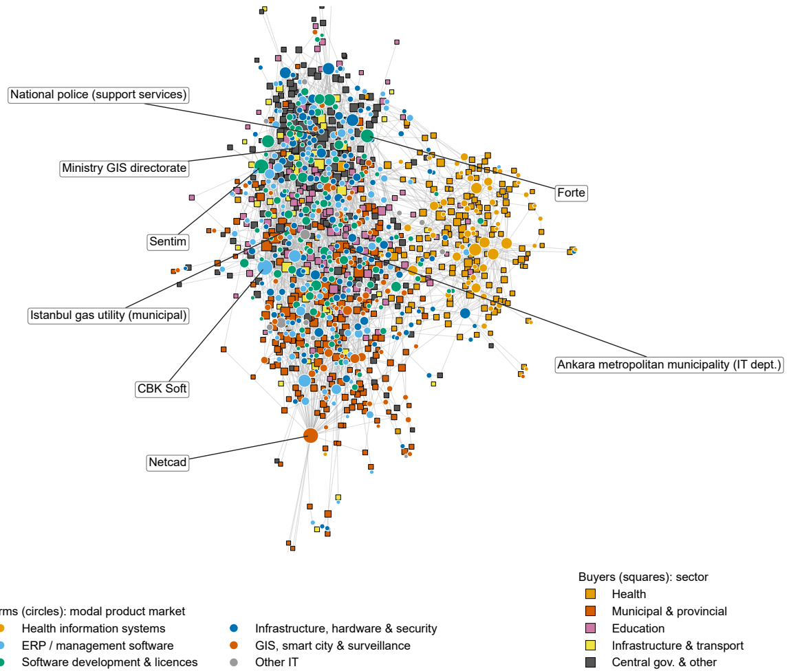
Figure S3: Core of the buyer-supplier network (nodes of degree \geq 3 , largest connected component; force-directed layout with fixed seed). Circles are firms coloured by their main product market; squares are buyers coloured by sector.
