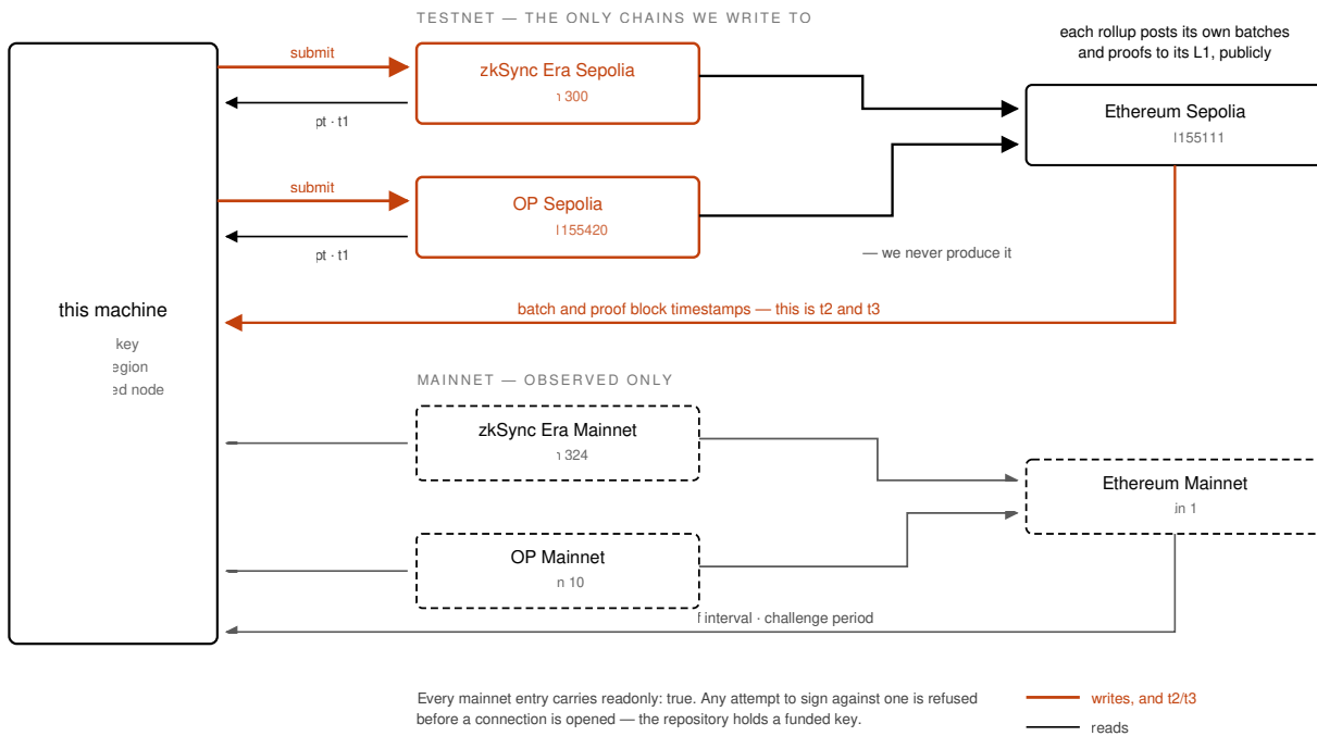
Figure 2. Six chains, two of which we write to. Everything else is read. The rollups publish their own batches and proofs to their L1 because their security depends on it; the study reads that evidence rather than producing any. Mainnet entries are flagged read-only and refuse a signature before a connection is even opened.
