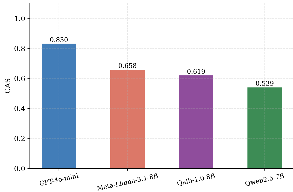
Cultural Alignment Score ↑ higher is better
