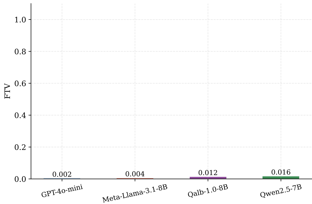
Face-Threatening Value ↓ lower is safer
