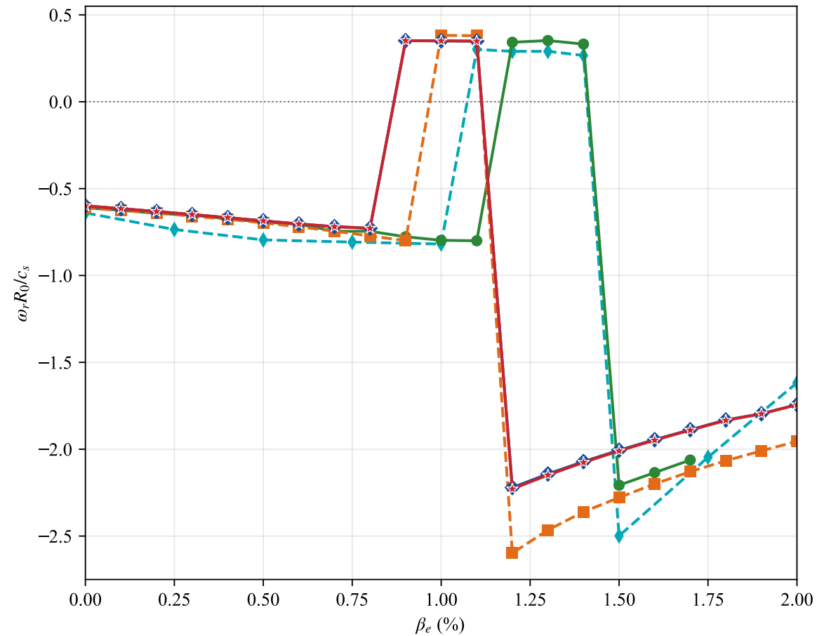
Xie et al. (2016) Figure 1: CBC electromagnetic benchmark
