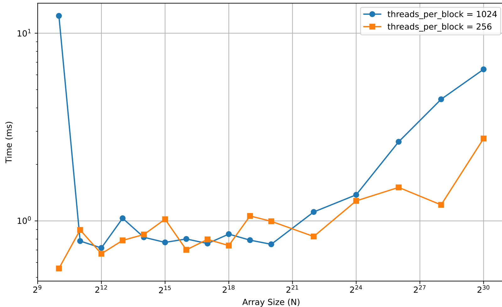
Parallel Reduction Performance
