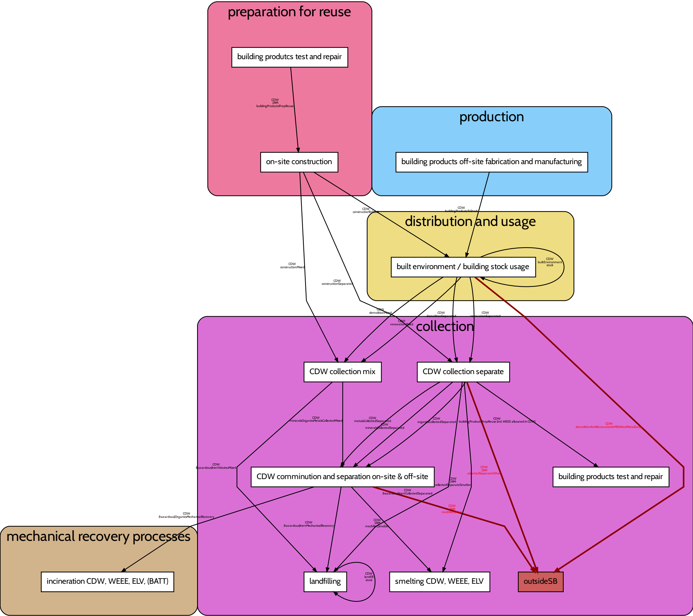
Flow chart for CDW: including models ['FutuRaM CDW', 'FutuRaM CDW/FutuRaM incineration', 'FutuRaM CDW/FutuRaM smelting']
